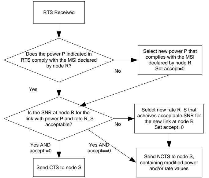
Fig. 4. Receiver R behavior
