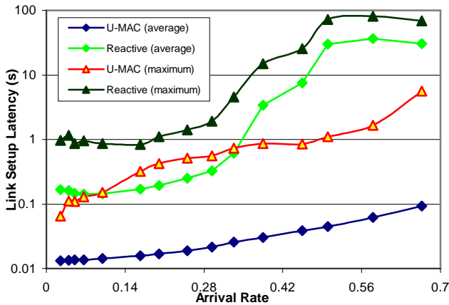
Fig. 9. Average Link Setup Latency vs Offered Load
