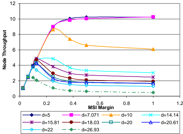
Fig. 6. Node Throughput vs. distance
