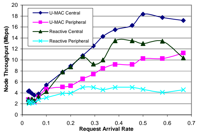
Fig. 14. Throughput of Central and Peripheral Nodes
