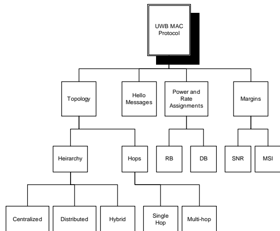
Fig. 1. Protocol Overview
