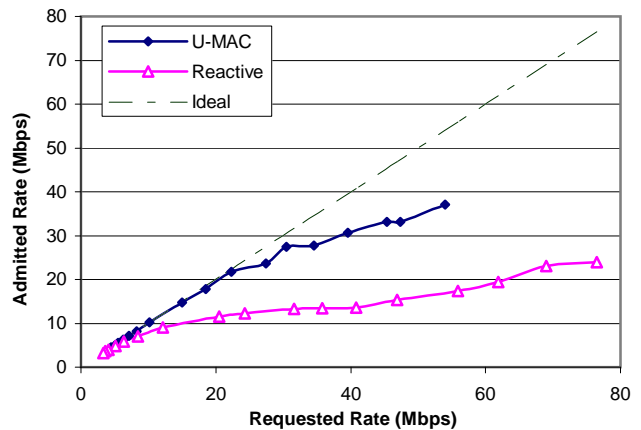
Fig. 11. Admitted Load vs Offered Load
