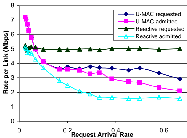
Fig. 13. Rate per Link vs Request Arrival Rate
