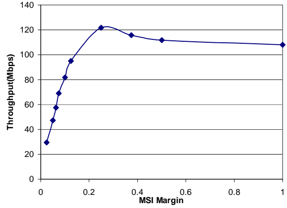
Fig. 8. Throughput vs. MSI Margin
