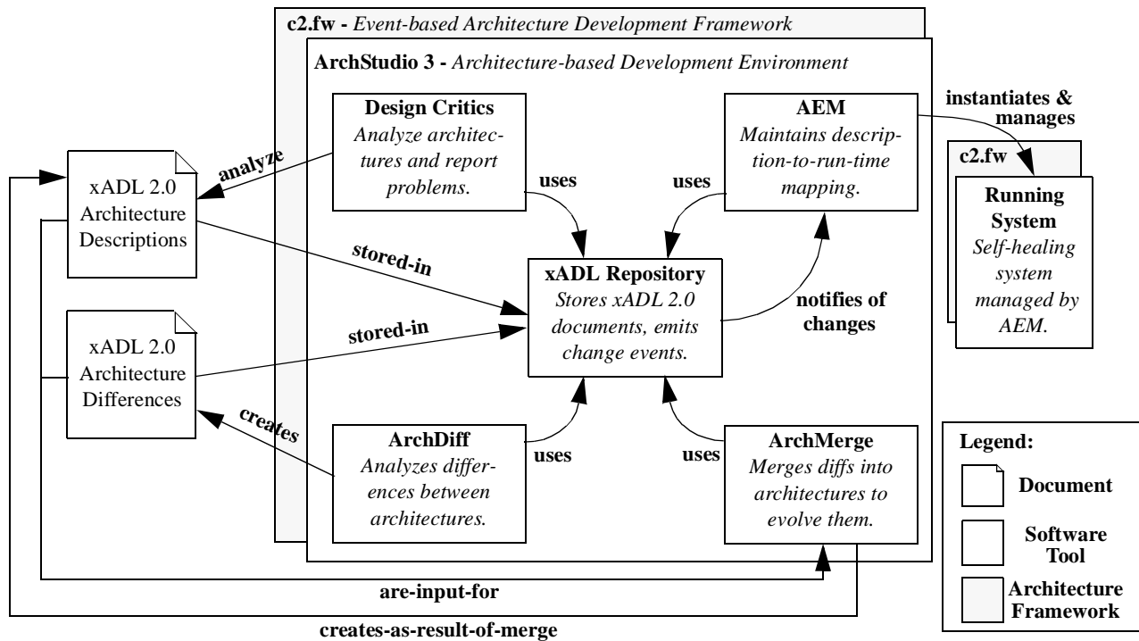
Fig. 1. Tools and documents found in our approach to self-healing systems and their relationships to each other.
