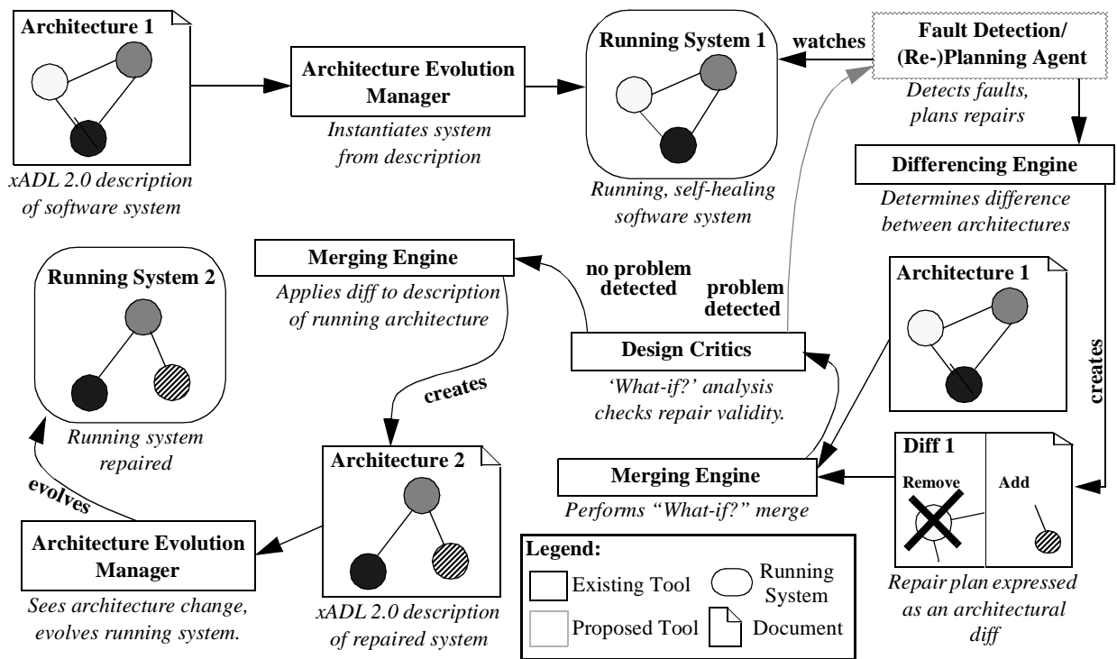
Fig. 2. Diagram showing the process steps of our approach, indicating completed tools and tools that we propose to build.
